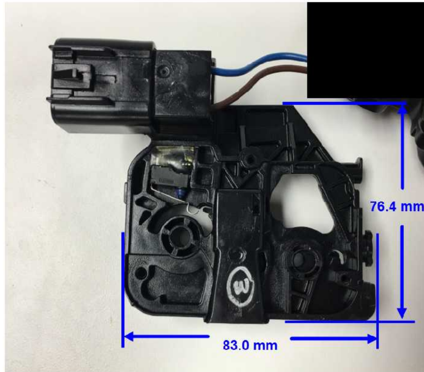
Top View
